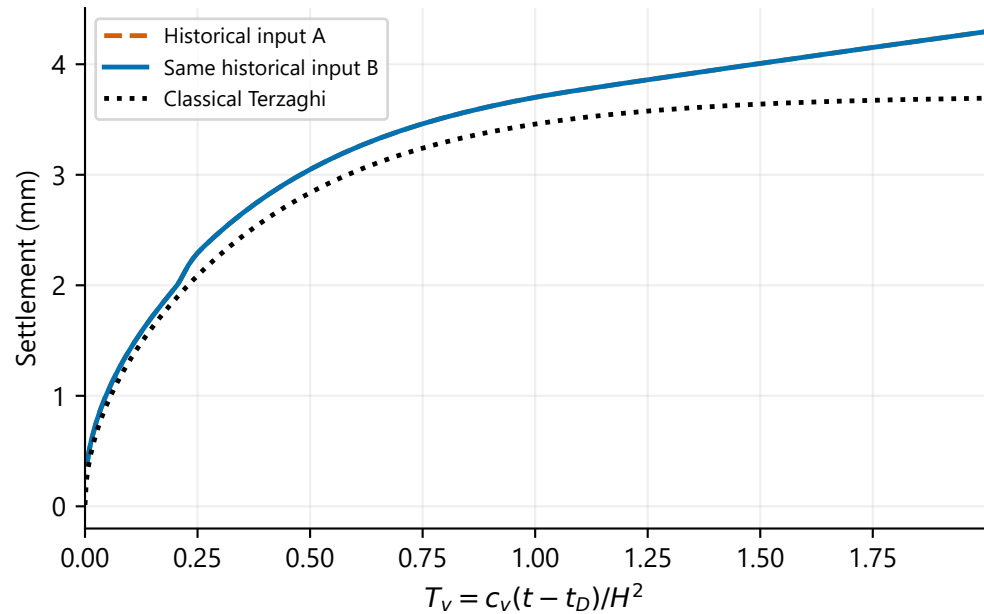
Top settlement
