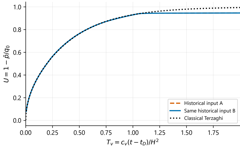
Consolidation degree
